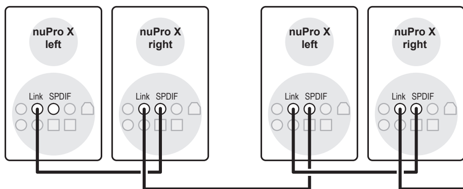
Use of more than two nuPro active loudspeakers
